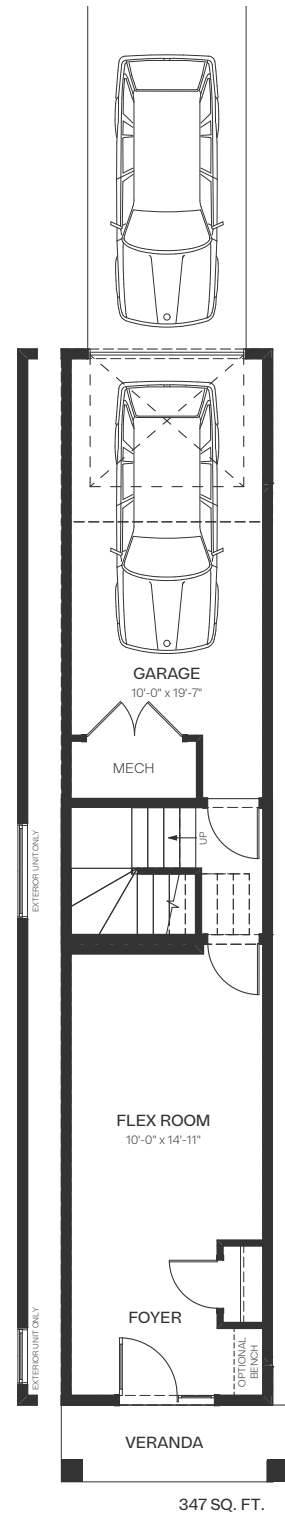
ground floor
